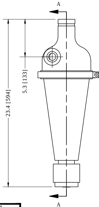
FRONT VIEW SCALE 1 / 6
