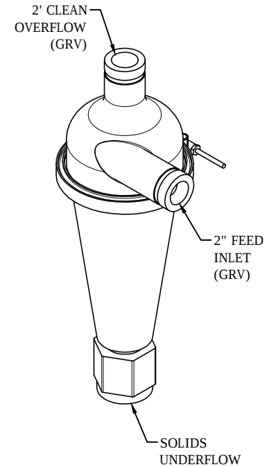
ISOMETRIC VIEW SCALE 1 / 6
